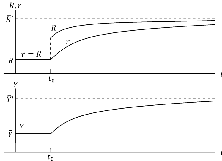
Figure 22.4: Time profiles of interest rates and output to an unanticipated shift in G (regime m ).
