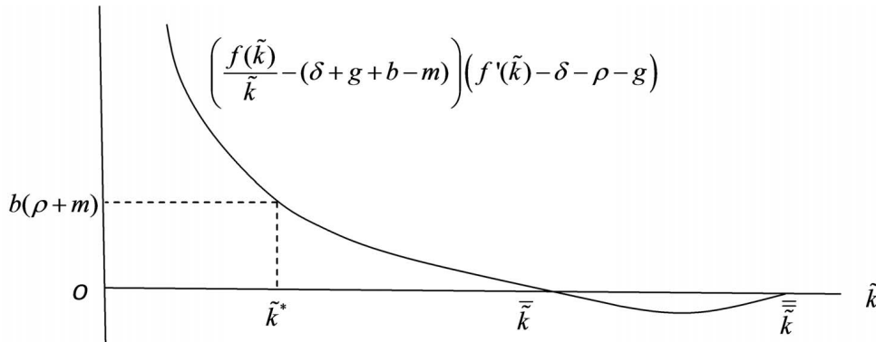
Figure 12.5: Existence of a unique \tilde{k}^* .
